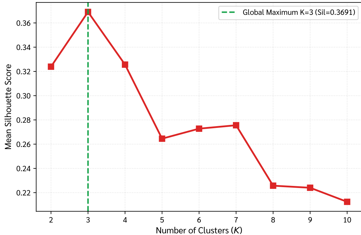
(b) Silhouette Coefficient on 5D PC Scores
