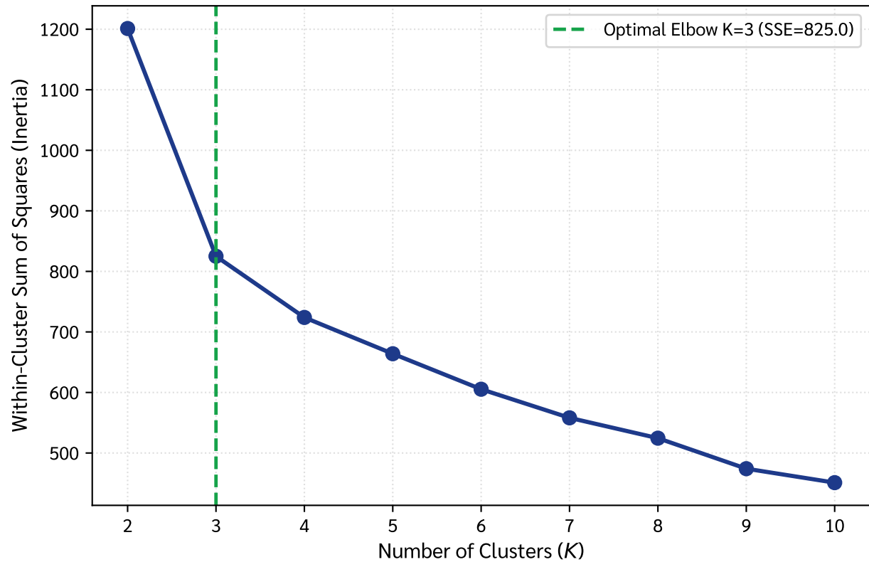
(a) Elbow Method on 5D PC Scores
